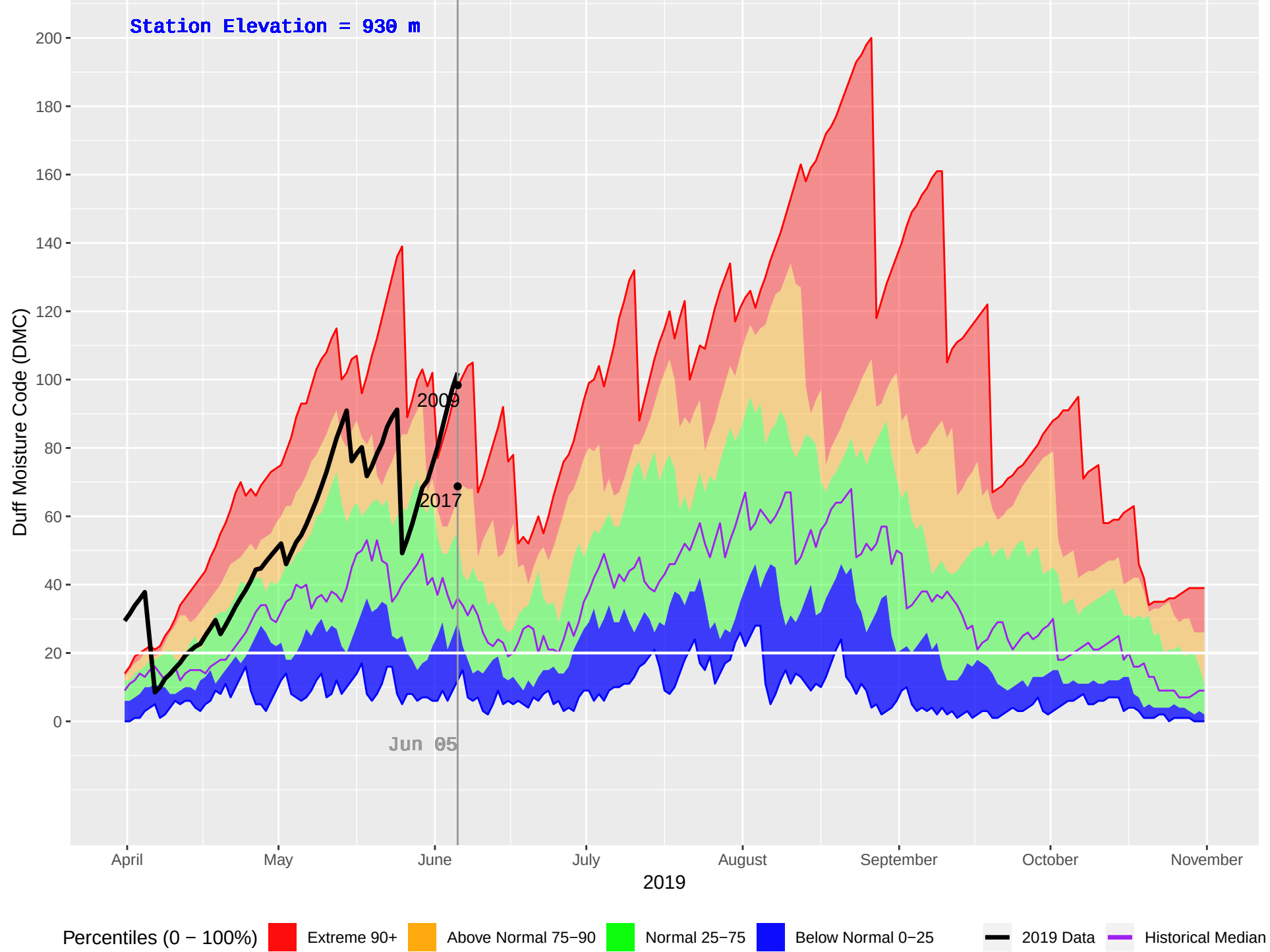
BRISCO (865) : Historical (2004–2018), Current (2019) Daily Duff Moisture Code (DMC)
