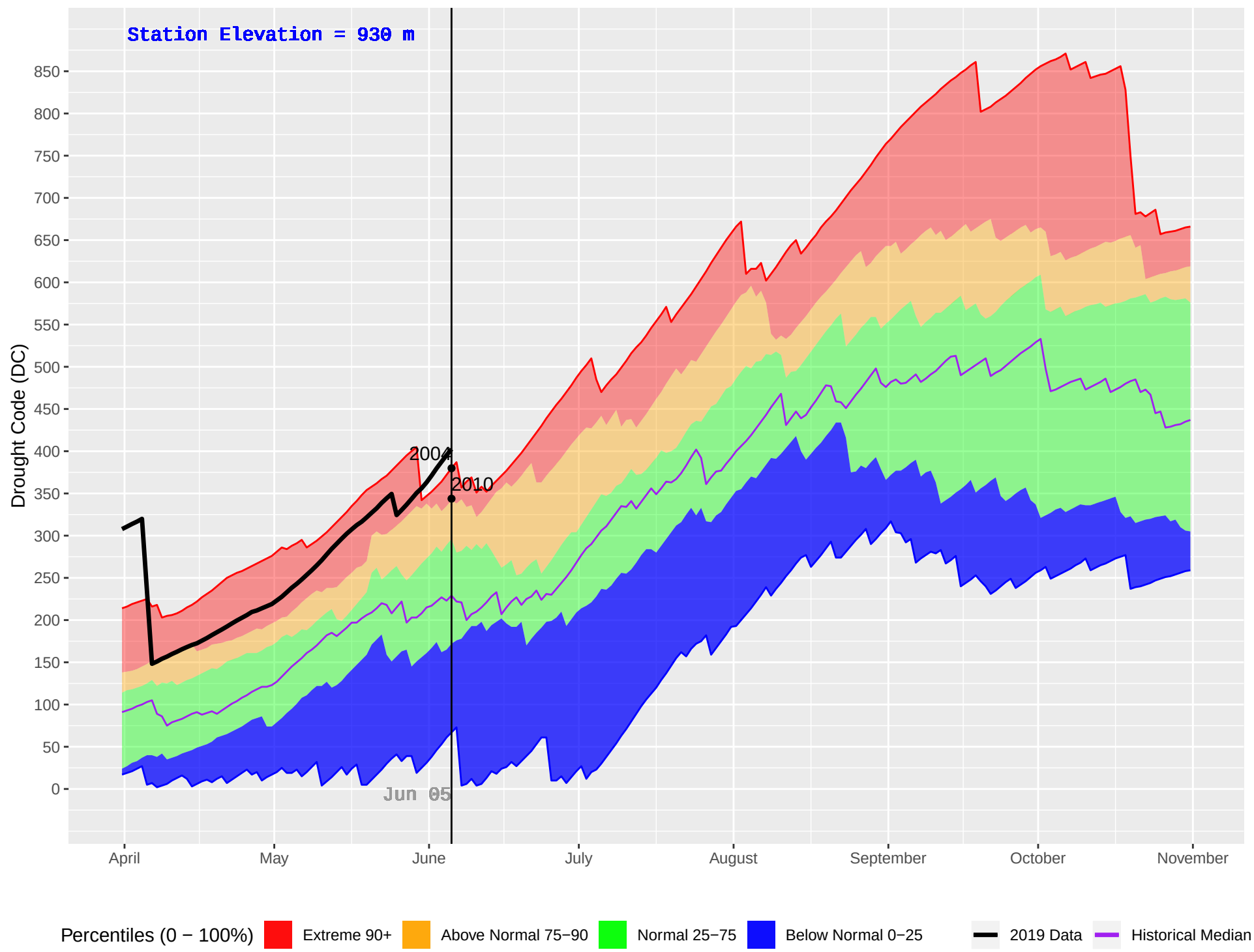
BRISCO (865) : Historical (2004–2018) and Current (2019) Daily Drought Code (DC)
