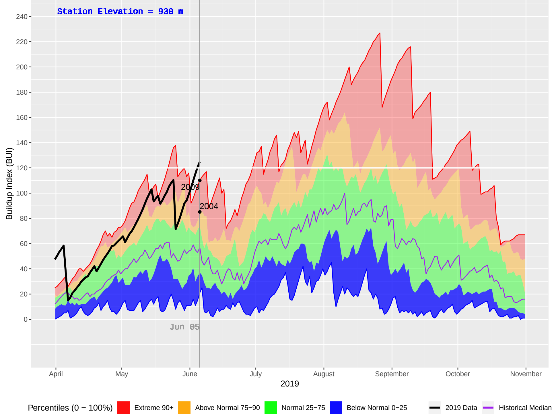
BRISCO (865) : Historical (2004–2018), Current (2019) Daily Buildup Index (BUI)
