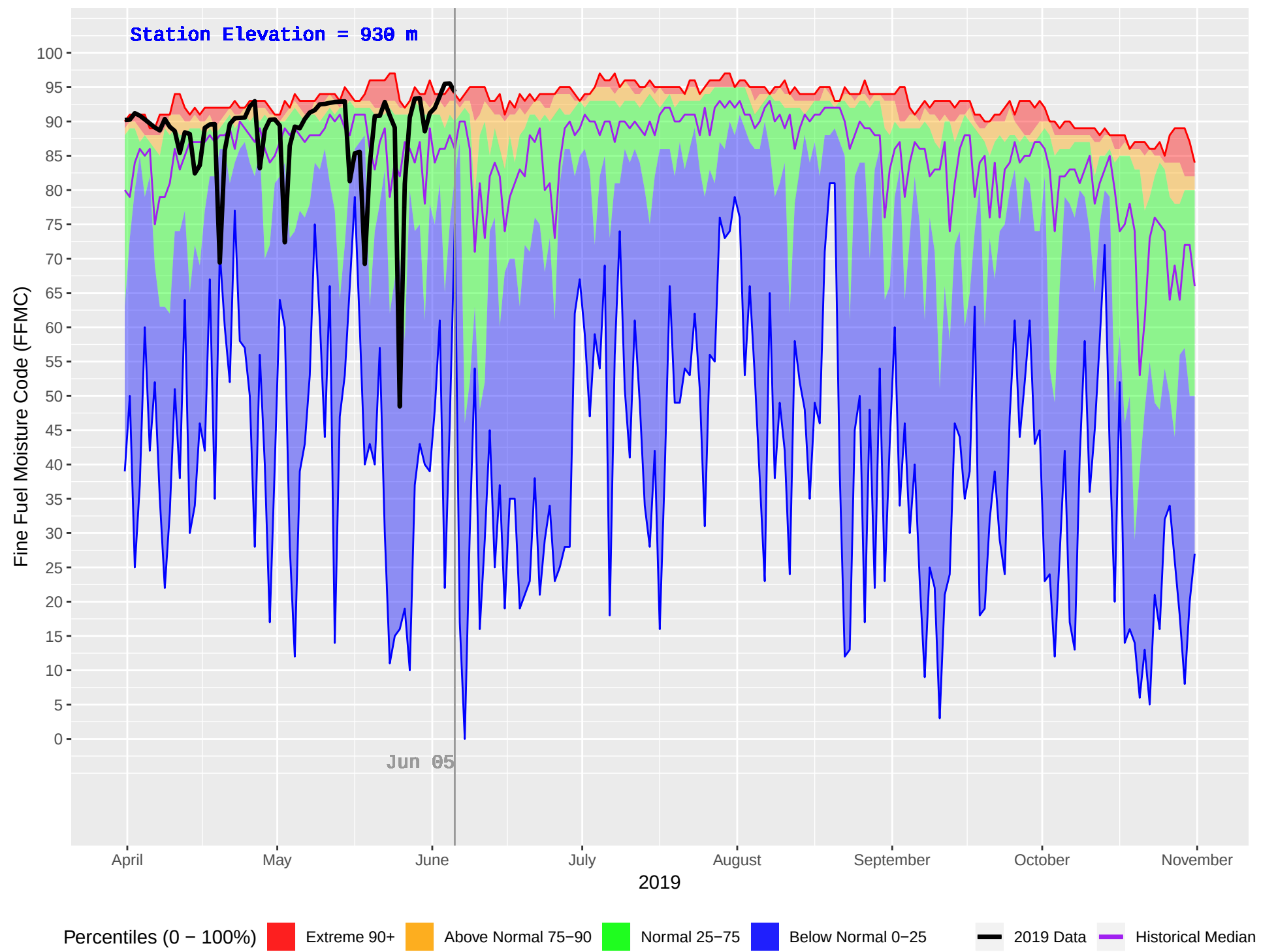
BRISCO (865) : Historical (2004–2018) and Current (2019) Daily Fine Fuel Moisture Code (FFMC)
