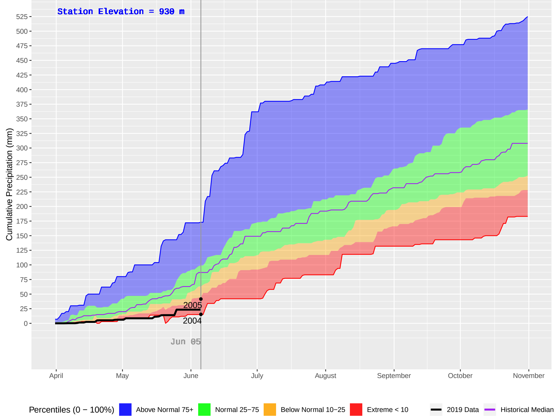
BRISCO (865) : Historical (2004–2018), Current (2019) Daily Cumulative Precipitation
