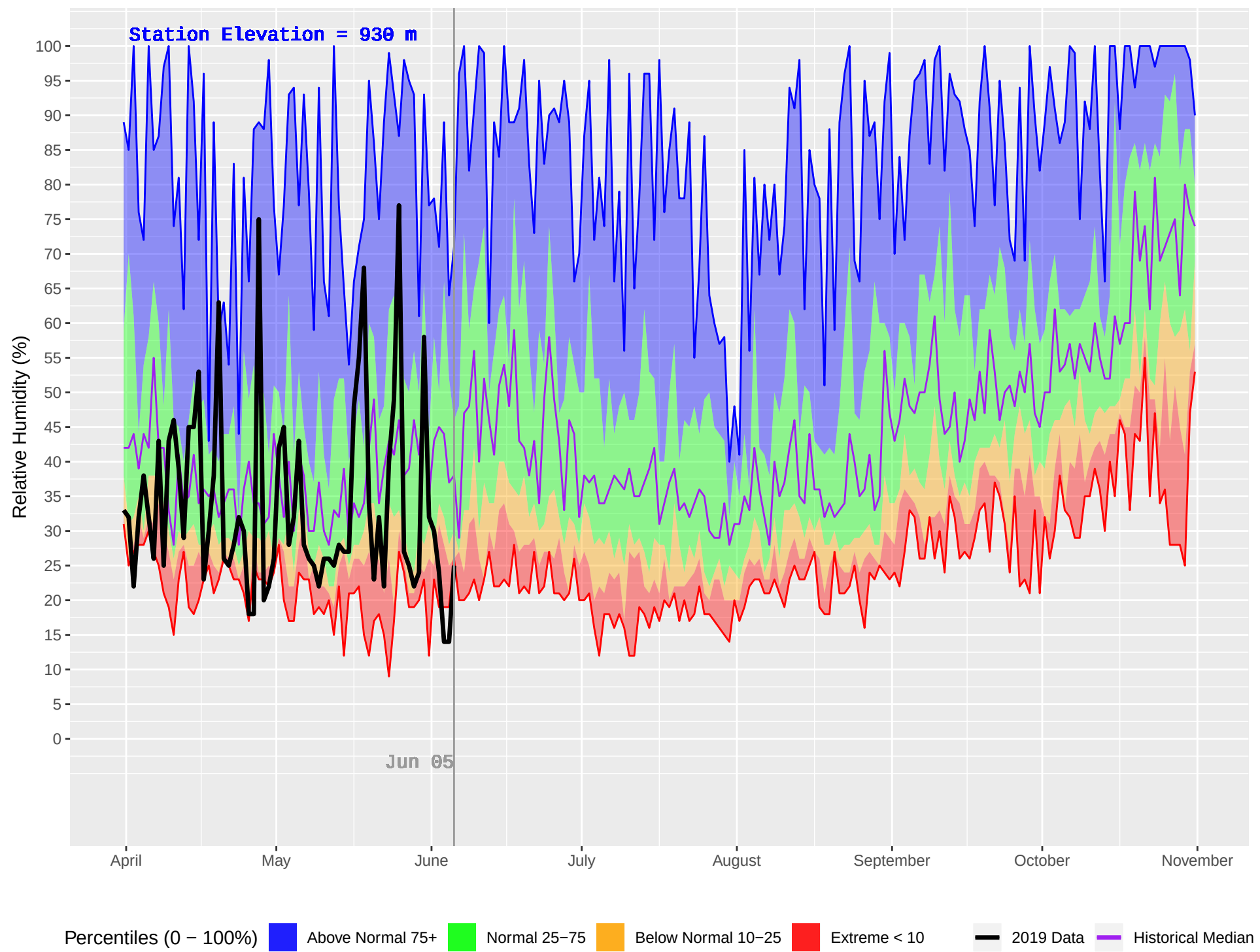
BRISCO (865) : Historical (2004–2018) and Current (2019) Daily Relative Humidity
