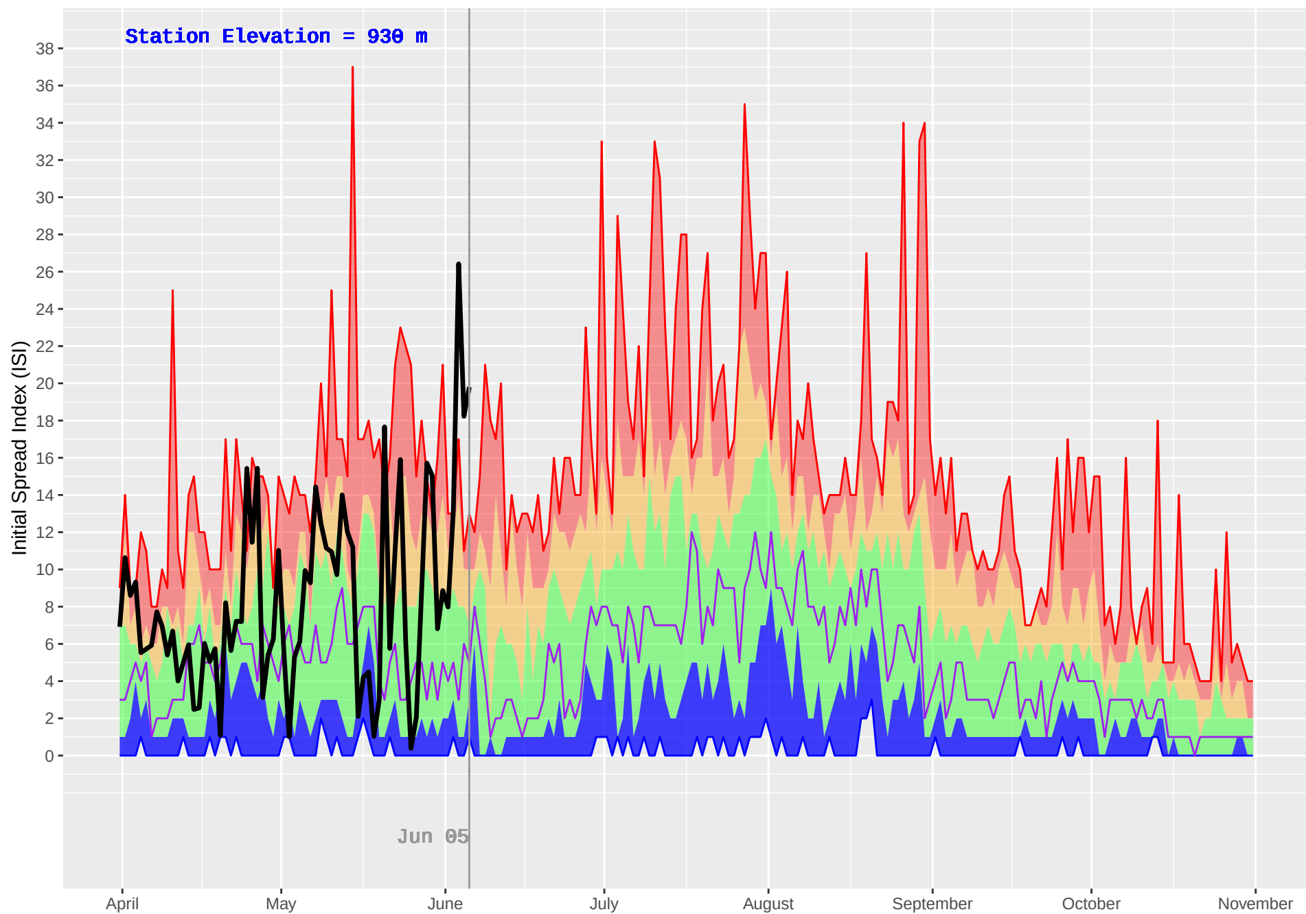
BRISCO (865) : Historical (2004–2018) and Current (2019) Daily Initial Spread Index (ISI)
