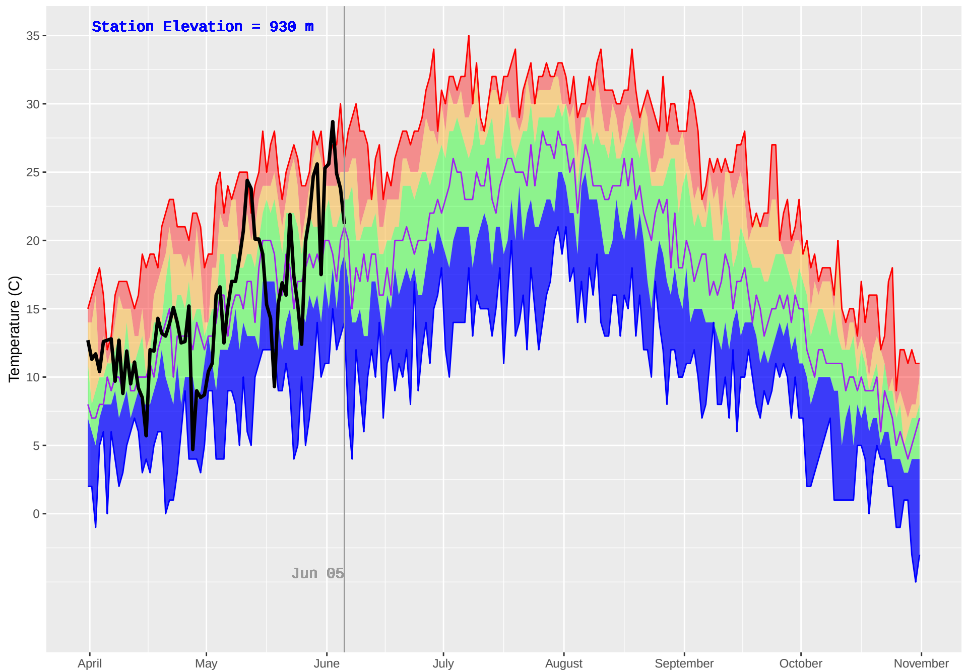
BRISCO (865) : Historical (2004–2018) and Current (2019) Daily Temperature
